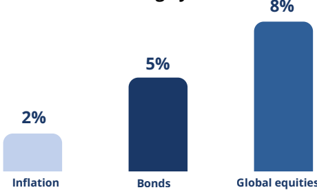
Average yield
