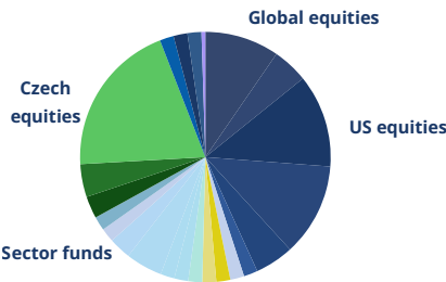
Model allocation
